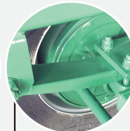
HEAVY DUTY SPRINGS 4"X2" (100X50MM) FOR UNRIVALED STABILITY (EXCLUSIVE TO SMYTH TRAILERS)
